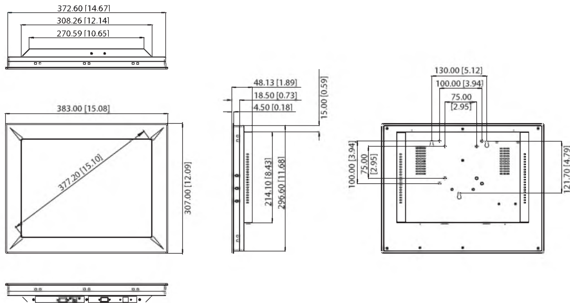
Panel Cut-out Dimensions: 374.6 x 298.6 mm (14.75" x 11.76")
